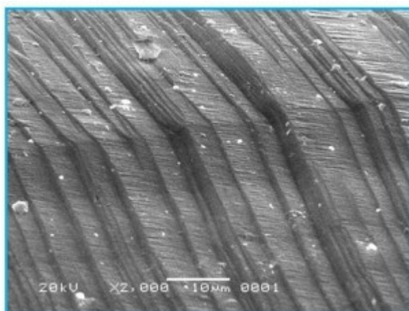
Figure 6: SEM image of completely grown brushite crystal at 10 \mu\text{m} .
